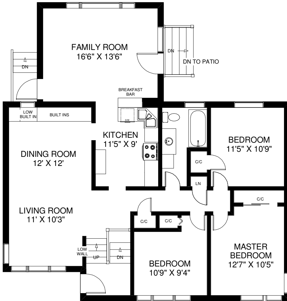
MAIN FLOOR APPROXIMATELY 1,400 SQ FT
