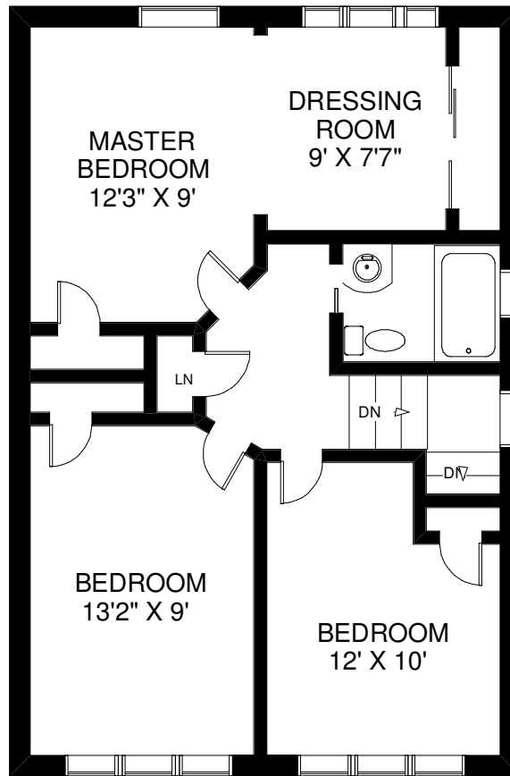
SECOND FLOOR APPROXIMATELY 650 SQ FT
