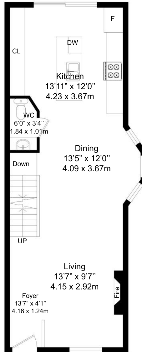
MAIN FLOOR 582 ft 2
