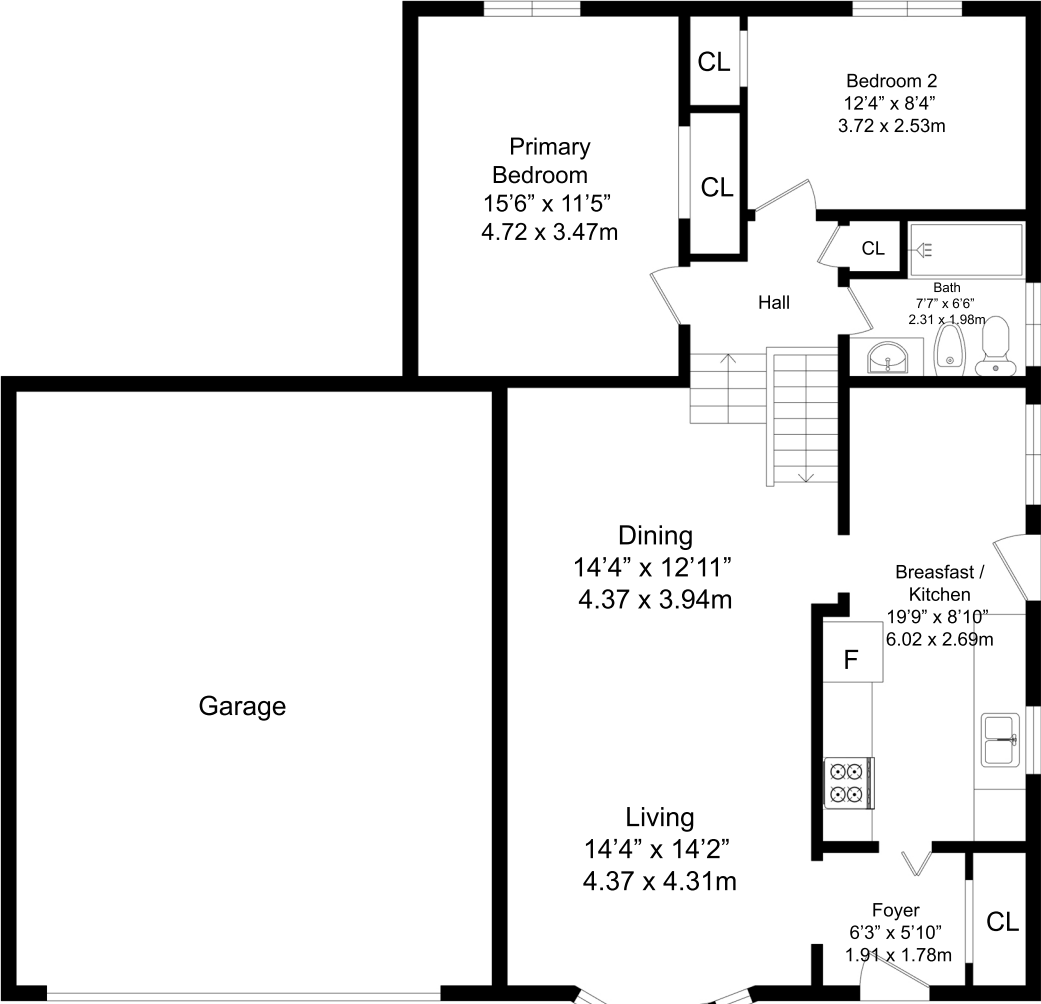
MAIN FLOOR 992 ft 2
