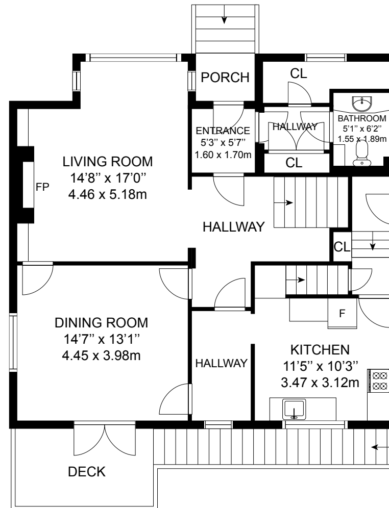
MAIN FLOOR
