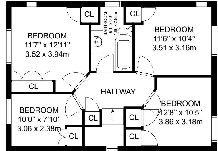
2ND FLOOR
