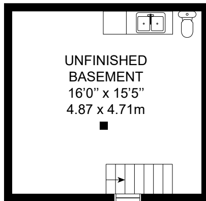
BASEMENT
