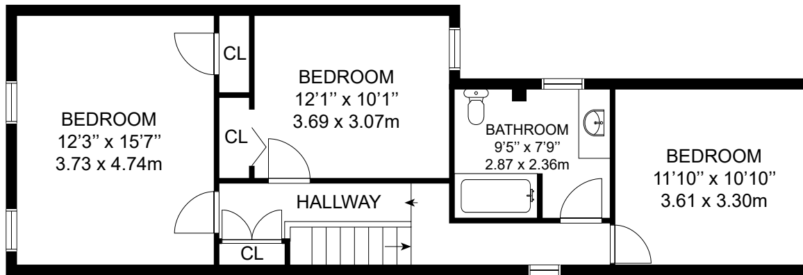
2ND FLOOR
