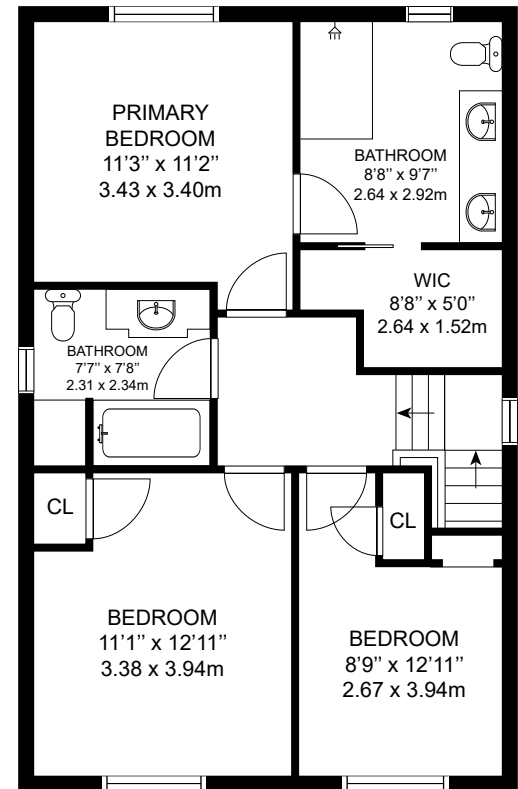
2ND LEVEL
