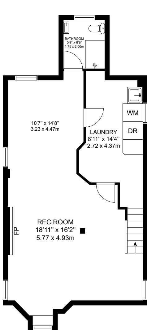
LOWER LEVEL
